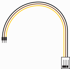
Switch connector
